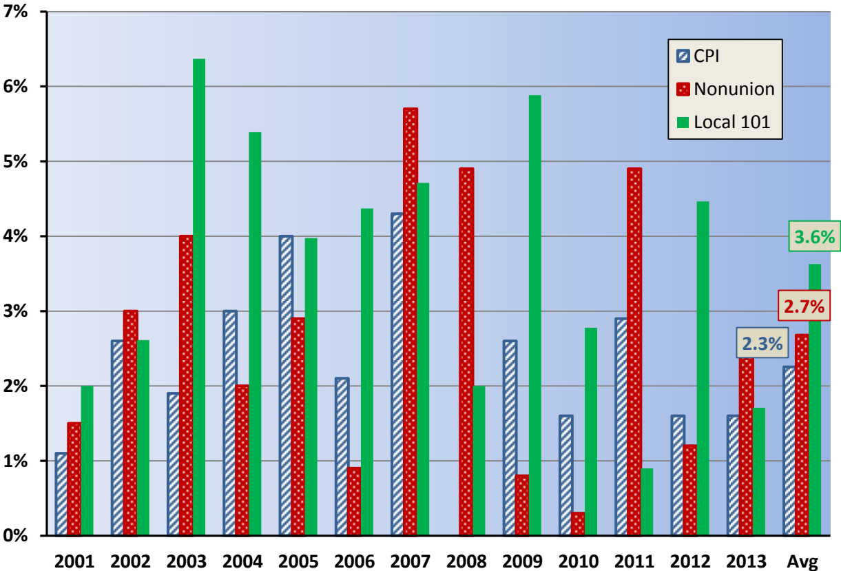
Exhibit 2 Annual Increase: Local 101 Compared to Benchmark Data
