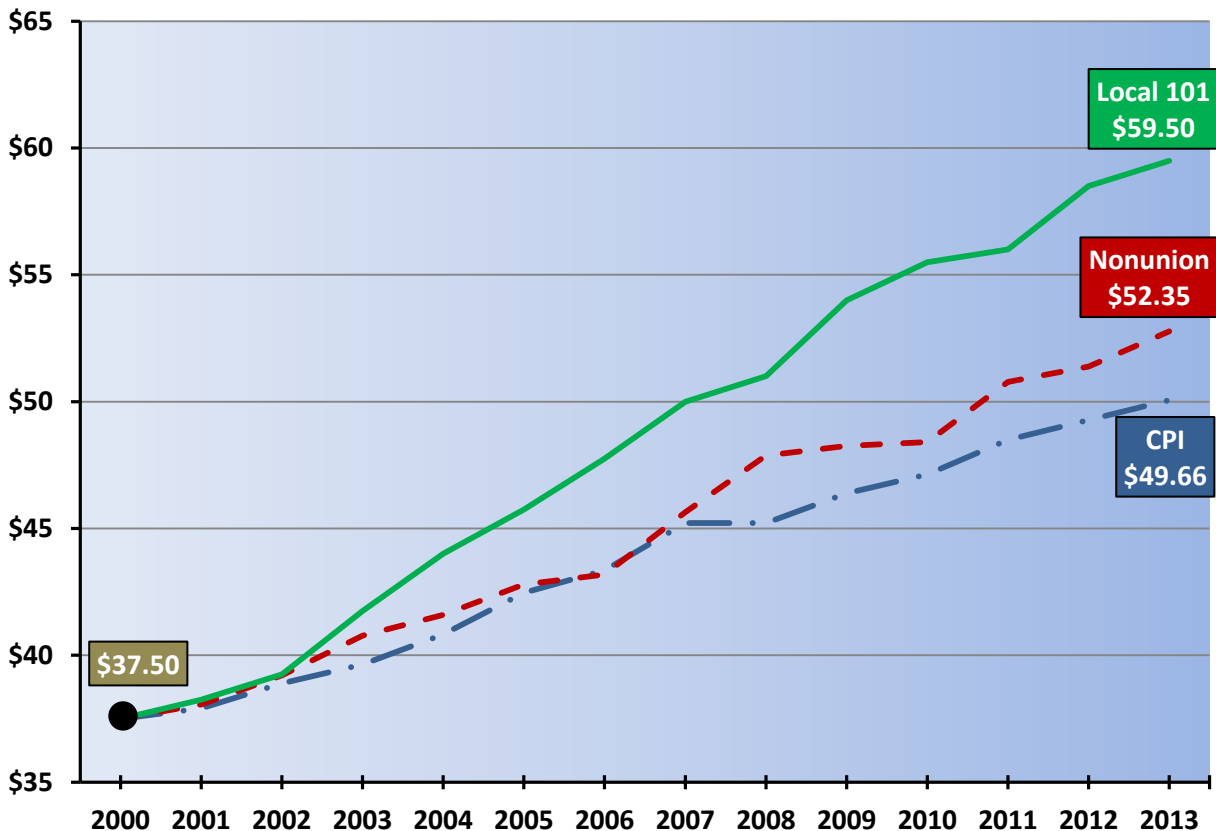
Wage and Fringe Benefits Growth: Local 101 Compared to Benchmark Data
