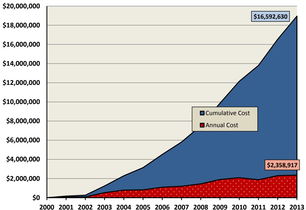
Cumulative Total Cost: Local 101 Based on the CPI
